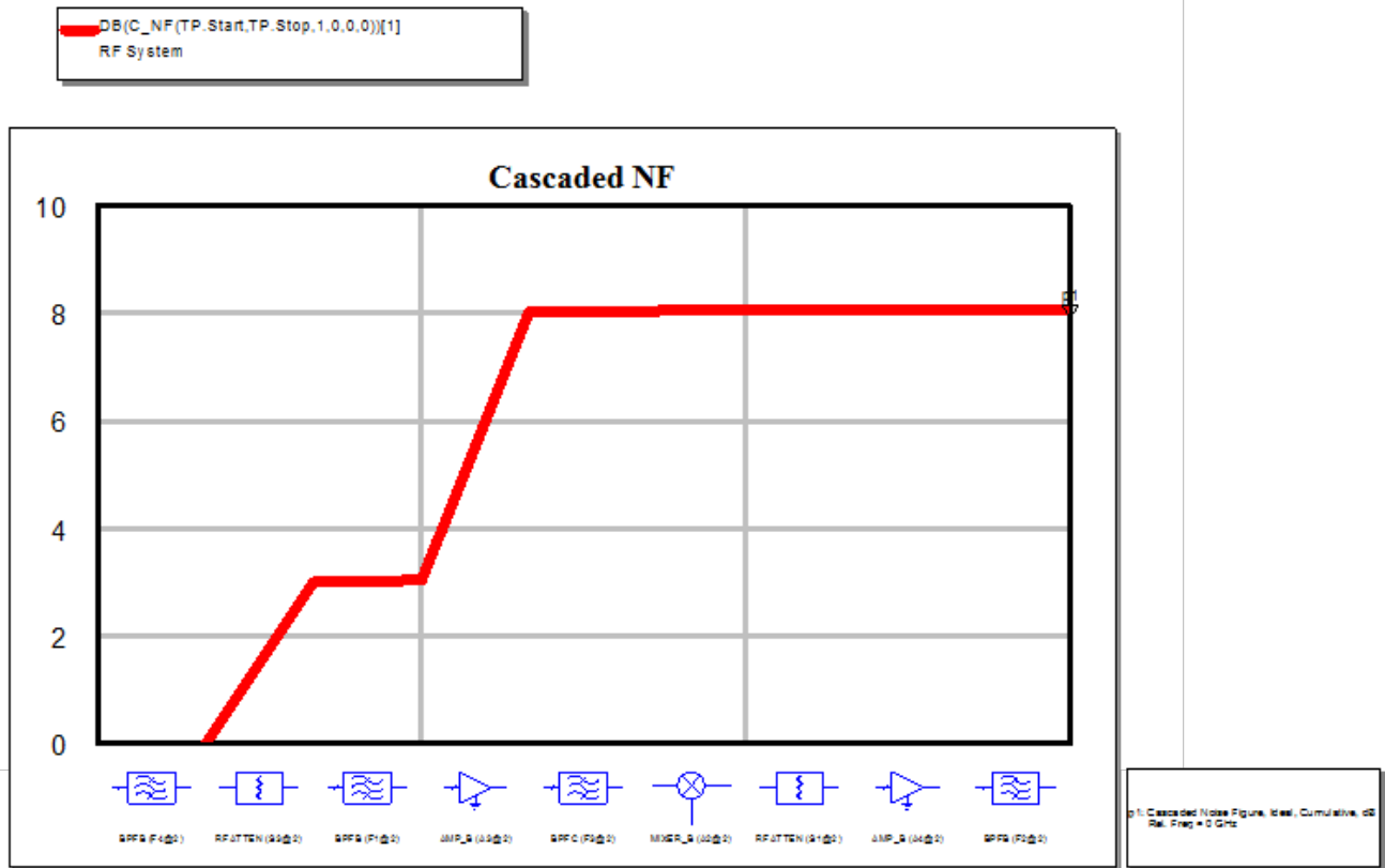
Graph - Cascaded NF over Frequency
